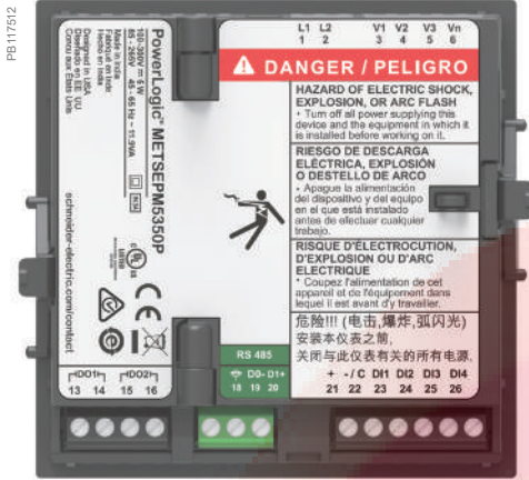
Rear view of PowerLogic PM5350P
