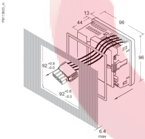
Dimensions PM5350PB
