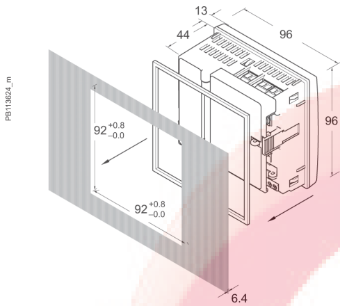
Dimensions PM5350IB
