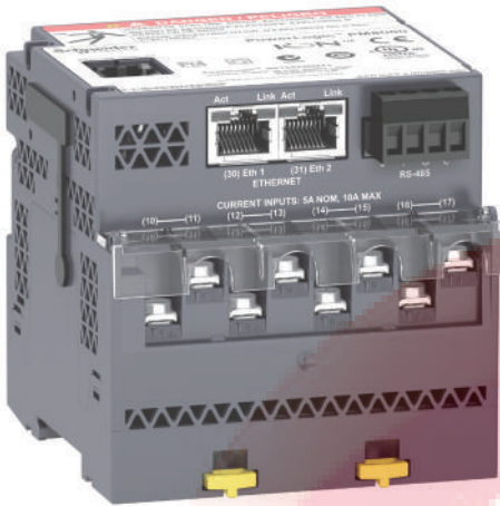
Underside of PM8000 meter (DIN rail version).
