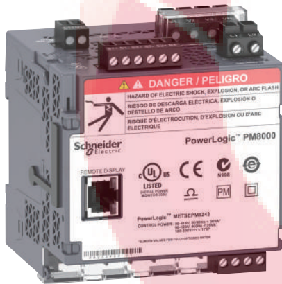
PowerLogic PM8000 series meter - rear view.
