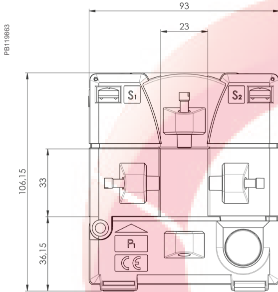
GA Dimensions
